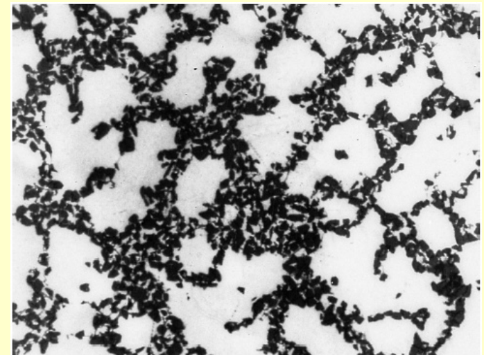
Microstructure of an aluminum casting alloy reinforced with silicon carbide particles.
