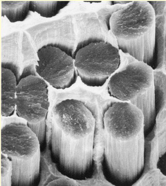
Scanning electron micrograph of the fracture surface of a silver-copper alloy reinforced with carbon fibers.
