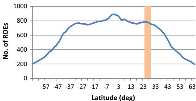
Fig. 12 Latitudinal variations of number of ROEs
