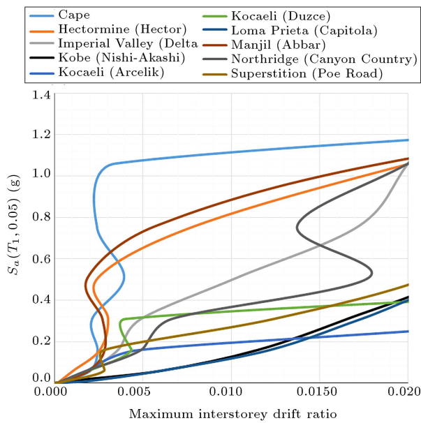
Figure 19. Incremental Dynamic Analysis (IDA) curves for 10-storey structure with e/L = 0.05 .
