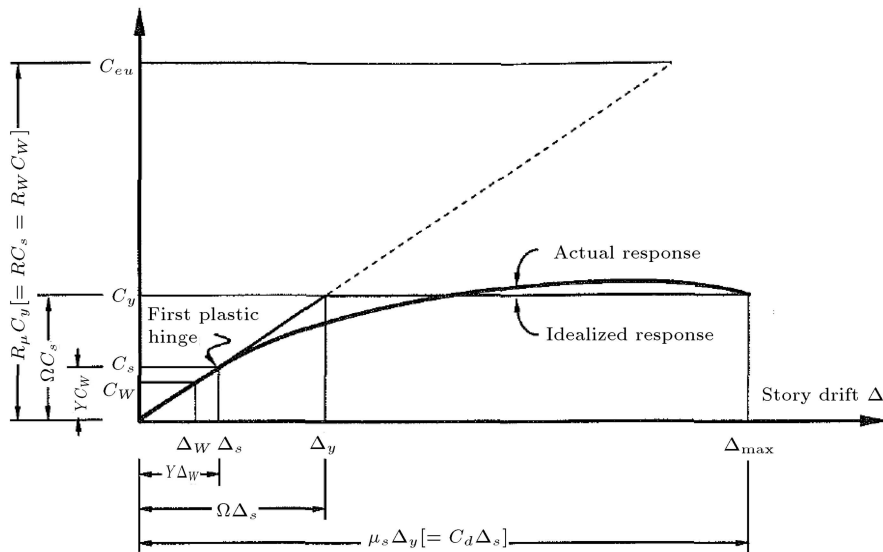
Figure 3. Elastic and inelastic responses of structure [30].
