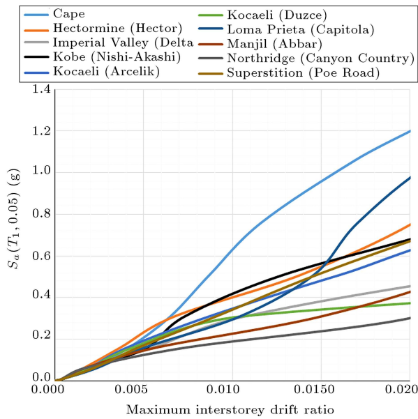
Figure 18. Incremental Dynamic Analysis (IDA) curves for 6-storey structure with e/L = 0.2 .
