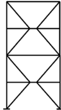
Figure 1. The arrangement of 2-storey eccentrically split-X bracing (ANSI/AISC 341-05) [28].
