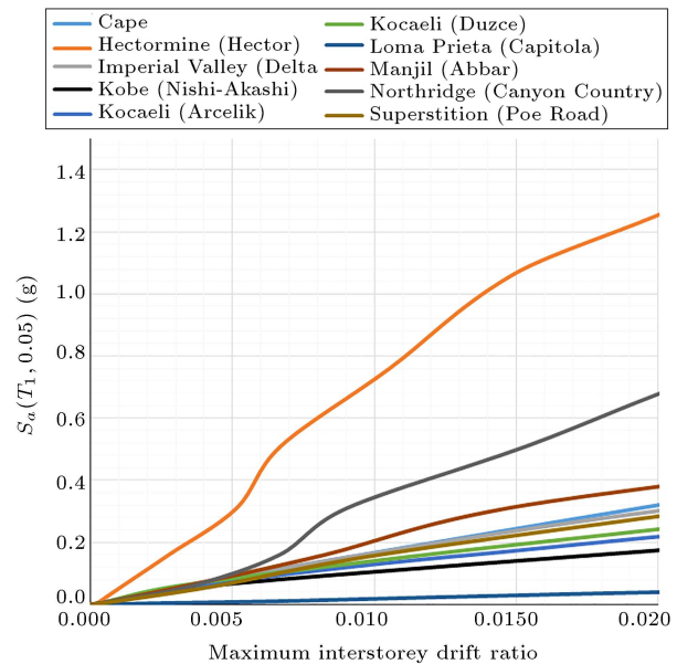
Figure 21. Incremental Dynamic Analysis (IDA) curves for 10-storey structure with e/L = 0.15 .
