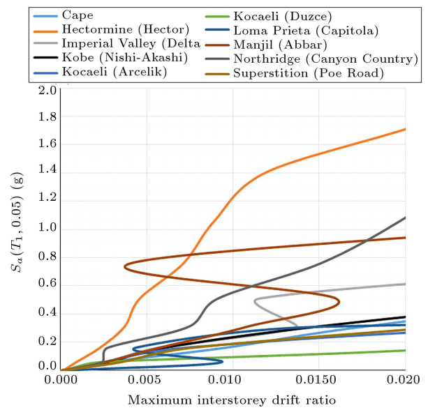
Figure 20. Incremental Dynamic Analysis (IDA) curves for 10-storey structure with e/L = 0.1 .
