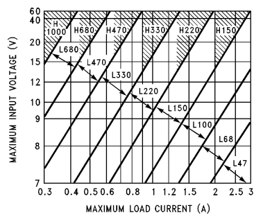
FIGURE 4. LM2576(HV)-5.0
