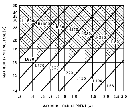
FIGURE 5. LM2576(HV)-12
