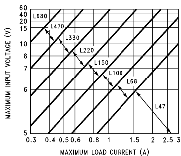
FIGURE 3. LM2576(HV)-3.3
